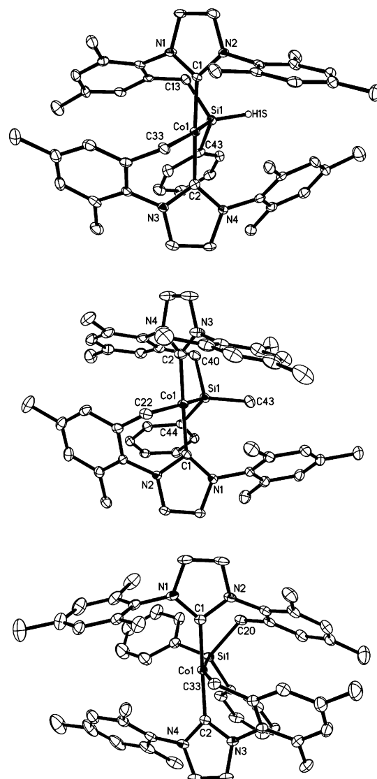
Figure 1. Molecular structures of 2a (top), 2b (middle), and 2c (bottom) showing 30% probability ellipsoids. Key bond distances [Å] and angles [ ^\circ ] for 2a : Co1–Si1 2.300(2), Co1–C33 2.048(5), Co1–C1 2.048(5), Co1–C2 1.891(5), Si1–Co1–C33 164.4(2) , C1–Co1–C2 178.3(2) ; for 2b : Co1–Si1 2.309(1), Co1–C22 2.067(2), Co1–C1 1.931(2), Co1–C2 1.912(2), Si1–Co1–C22 160.6(1) , C1–Co1–C2 174.3(1) ; for 2c : Co1–Si1 2.327(1), Co1–C33 2.070(2), Co1–C1 1.900(2), Co1–C2 1.907(2), Si1–Co1–C33 161.7(1) , C1–Co1–C2 176.3(1) .
