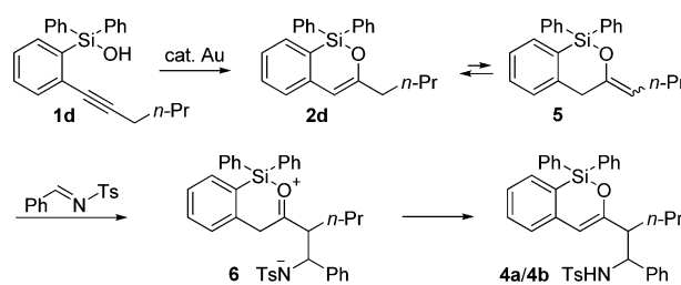
Scheme 3. Plausible Mechanism of the Tandem Hydrosilyloxylation/Isomerization/Mannich Reaction
