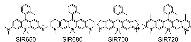
Figure 1. Chemical structures of SiR650 and newly synthesized NIR wavelength-excitable fluorescence dyes, SiR-NIRs.
