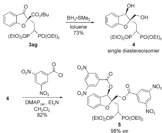
Scheme 1. Reduction of bisphosphonate \beta -ketoester 3ag to diol 4 and subsequent benzoylation to 5 .
