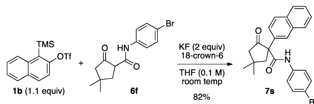
Scheme 2. Regioselective \alpha -Arylation
