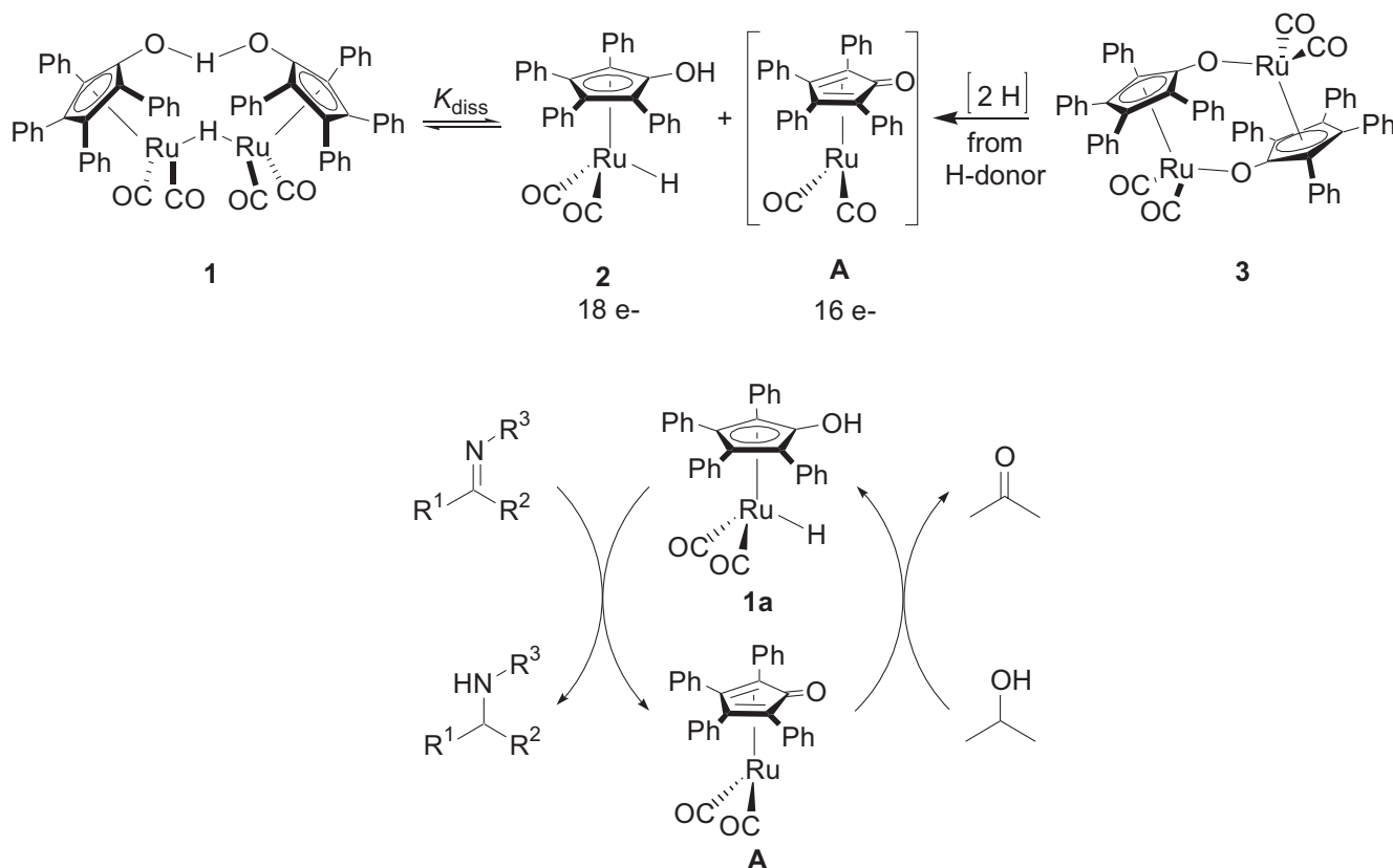
Fig. 1. Comparison between precatalysts 1 and 3 in the transfer hydrogenation of imine 6 in toluene- d_8 at 70 °C with isopropanol- d_8 using 0.6 mol% catalyst. The conversion was measured by ^1\text{H} NMR.
