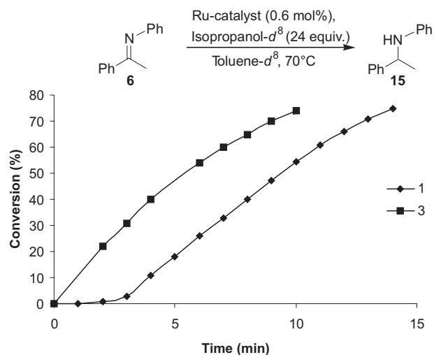
Fig. 1. Comparison between precatalysts 1 and 3 in the transfer hydrogenation of imine 6 in toluene- d_8 at 70 °C with isopropanol- d_8 using 0.6 mol% catalyst. The conversion was measured by ^1\text{H} NMR.
