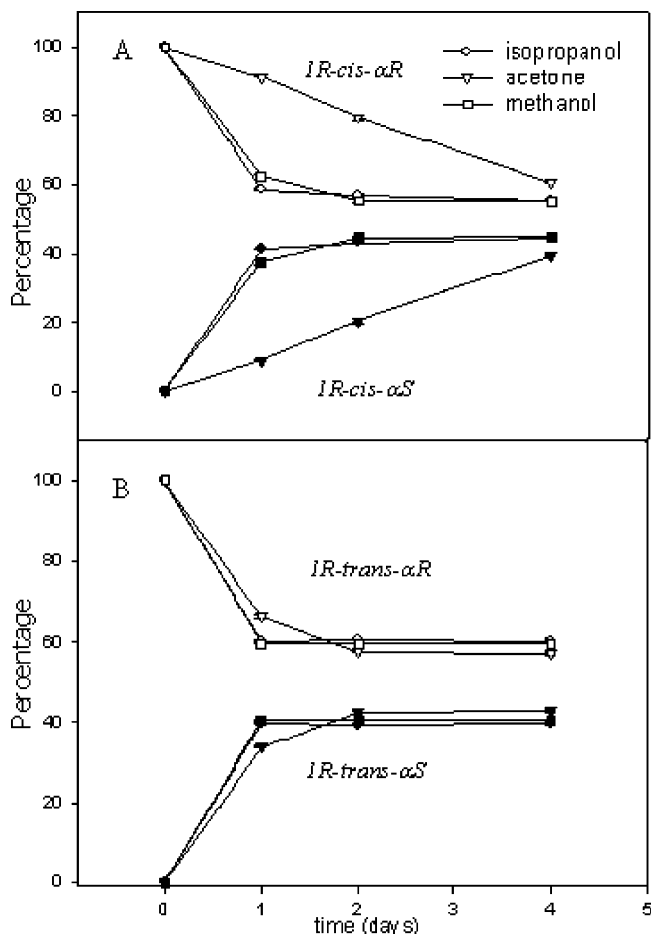
Figure 4. Disappearance of the starting enantiomer and appearance of the converted enantiomer of CP as a function of time in solvent–water mixtures (1:1, v/v). (A) Enantiomerization of 1 R -cis- \alpha R to 1 R -cis- \alpha S and (B) enantiomerization of 1 R -trans- \alpha R to 1 R -trans- \alpha S. Open dots refer to starting enantiomer, and solid dots refer to converting enantiomer.
