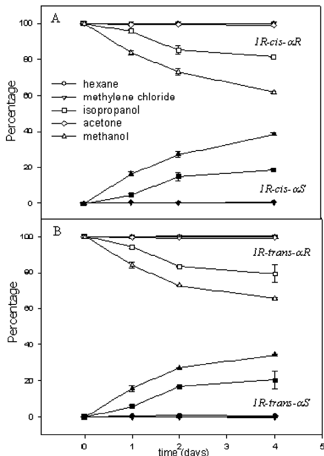
Figure 3. Disappearance of the starting enantiomer and appearance of the converted enantiomer of CP as a function of time in selected organic solvents. (A) Enantiomerization of 1R-cis-αR to 1R-cis-αS and (B) enantiomerization of 1R-trans-αR to 1R-trans-αS. Open dots refer to starting enantiomer, and solid dots refer to converting enantiomer.
