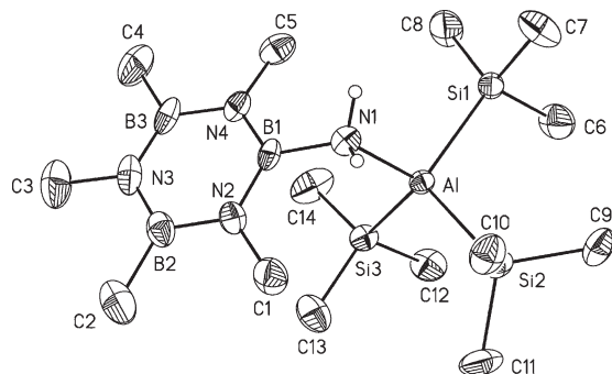
Figure 1. Molecular structure and atom numbering scheme for 1 · ( \text{Me}_3\text{B}_3\text{N}_3\text{Me}_3 ) 0.5 . The solvate molecule \text{Me}_3\text{B}_3\text{N}_3\text{Me}_3 is not shown.
