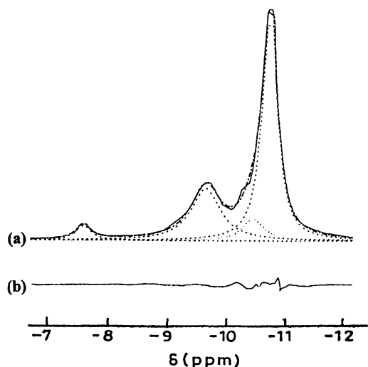
Fig. 3. (a) Partial ^{29}\text{Si} -NMR spectrum of 1 depicting carbosilyl region; — spectrum, --- calculated spectrum; .... deconvoluted peaks. (b) Difference spectrum of the actual and calculated spectrum.
