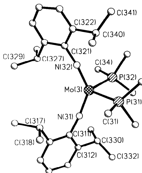
Fig. 1. Molecular structure of the unique molecule of [\text{Mo}(\text{N-2,6-}^i\text{Pr}_2\text{C}_6\text{H}_3)_2(\text{PMe}_3)_2] ( 1 ). Key dimensions: Mo(3)–P(31) 2.400(4) , Mo(3)–P(32) 2.405(5) , Mo(3)–N(31) 1.805(13) , Mo(3)–N(32) 1.797(10) Å; P(31)–Mo(3)–N(31) 98.9(3) , P(31)–Mo(3)–N(32) 110.1(3) , P(32)–Mo(3)–P(31) 96.9(2) , P(32)–Mo(3)–N(31) 109.0(4) , P(32)–Mo(3)–N(32) 98.5(4) , N(31)–Mo(3)–N(32) 137.1(5) , Mo(3)–N(31)–C(311) 169.8(9) , Mo(3)–N(32)–C(321) 172.3(9)^\circ .
