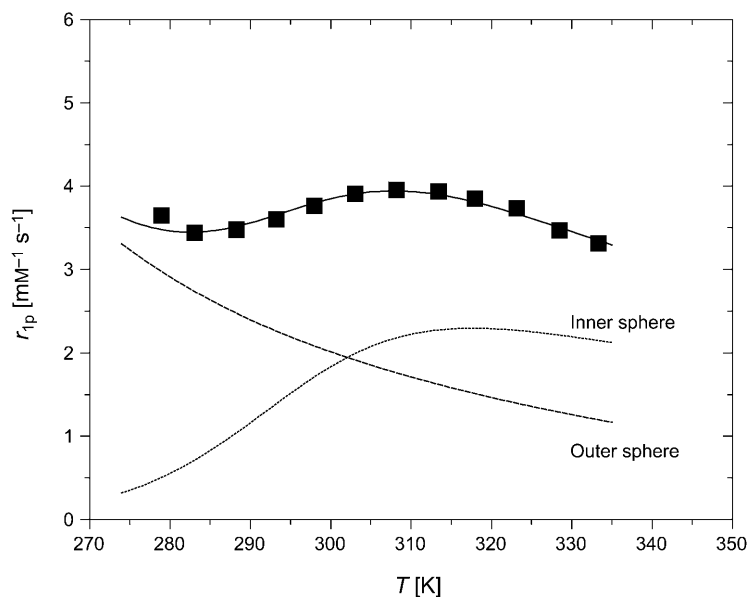
Fig. 4. Temperature dependence of the ^1\text{H} relaxivity r_{1p} for [\text{Gd}(\text{L1})] at 20 MHz and pH 7.2. The solid line through the data points (■) represents the best result of the fitting to the experimental data (see Table); the calculated inner- and outer sphere contributions to the relaxivity are also represented.
