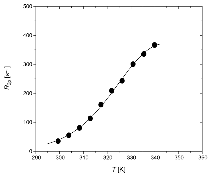
Fig. 3. Plot of the paramagnetic contribution to the ^{17}\text{O} transverse relaxation rate R_{2p} as a function of temperature at 9.4 T (12.2 MHz) and neutral pH for a 10.9 mM aqueous solution of [\text{Gd}(\text{L1})]
