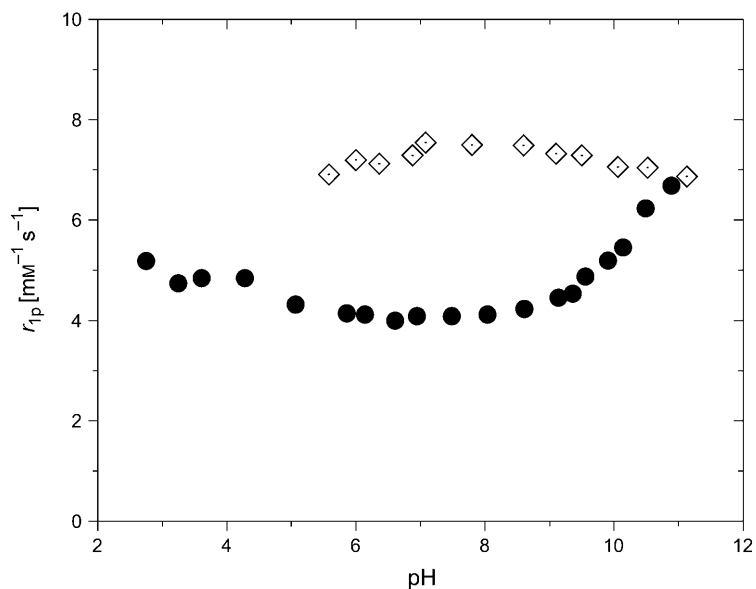
Fig. 1. Plot of H -atom relaxivity r_{1p} at 20 MHz and 298 K vs. pH for [\text{Gd}(\text{L1})] (●) and [\text{Gd}(\text{L2})] (◇)
