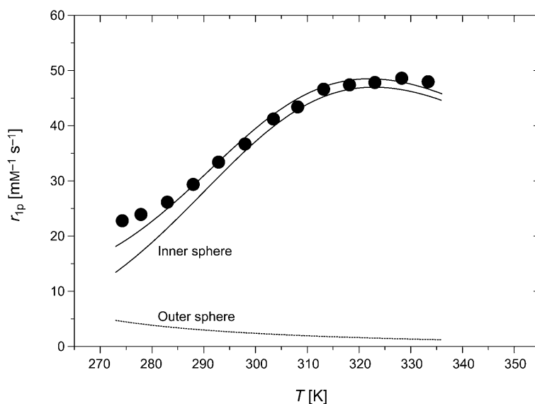
Fig. 7. Variable-temperature ^1\text{H} -NMR relaxation data (relaxivity r_{1p} ) for [\text{Gd}(\text{L2})] at 20 MHz and at a concentration above the cmc (0.25 mM), normalized to 1 mM concentration of Gd. The solid line through the data points (●) represents the best result of the fitting to the experimental data (see the Table); the calculated inner- and outer-sphere contributions to the relaxivity are also represented.
