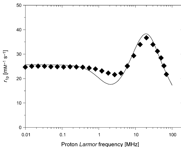
Fig. 6. ^1\text{H} -NMRD profile (relaxivity r_{1p} vs. ^1\text{H} Larmor frequency) of [\text{Gd}(\text{L2})] at pH 7.2 and 298 K at a concentration above the cmc (0.3 mM). The solid curve through the data points is calculated with the parameters reported in the Table.
