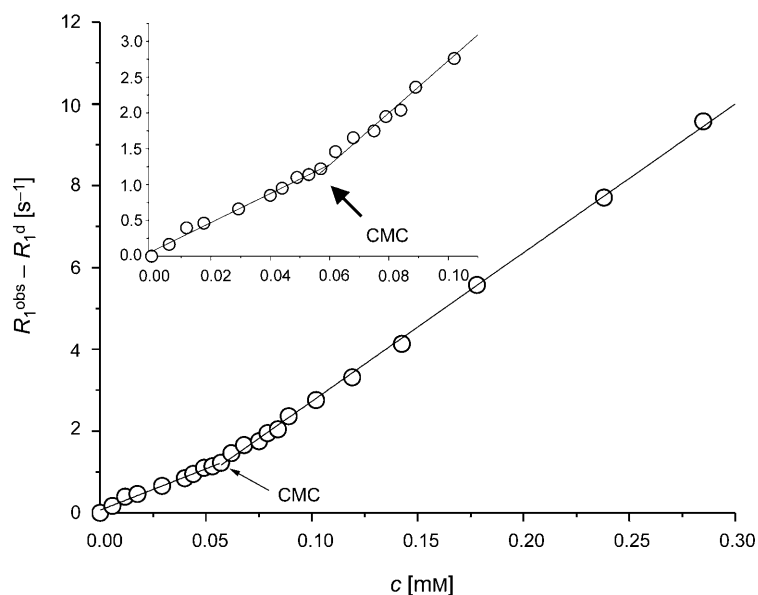
Fig. 5. Plot of the \text{H}_2\text{O} ^1\text{H} longitudinal relaxation rate at 20 MHz and 298 K as a function the total \text{Gd}^{\text{III}} concentration for [\text{Gd}(\text{L}2)] and least-squares fit according to Eqn. 2
