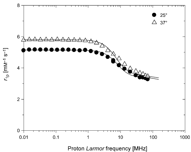
Fig. 2. ^1\text{H} -NMRD Relaxation data (relaxivity r_{1p} vs. ^1\text{H} Larmor frequency) for [\text{Gd}(\text{L1})] at pH 7.2 and 298 K ( \Delta ) and 310 K ( \bullet ). The solid lines represent the best results of the fitting to the experimental points (see Table).
