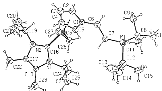
Fig. 3. Structure of 16 in the crystal. Selected bond lengths (Å) and angles ( ^\circ ): Co1–C1 2.07(2), Co1–C2 2.03(2), Co1–C3 2.07(2), Co1–C4 2.04(2), Co1–C5 2.08(2), Co1–C16 1.929(8), Co1–C27 1.97(2), Co1–C28 1.91(2), C16–N1 1.39(2), C16–N2 1.35(2), C27–C28 1.355(13), Co1–C27–C28 67.2(13), Co1–C28–C27 71.9(13), C27–Co1–C16 91.6(6), C28–Co1–C16 95.2(7)
