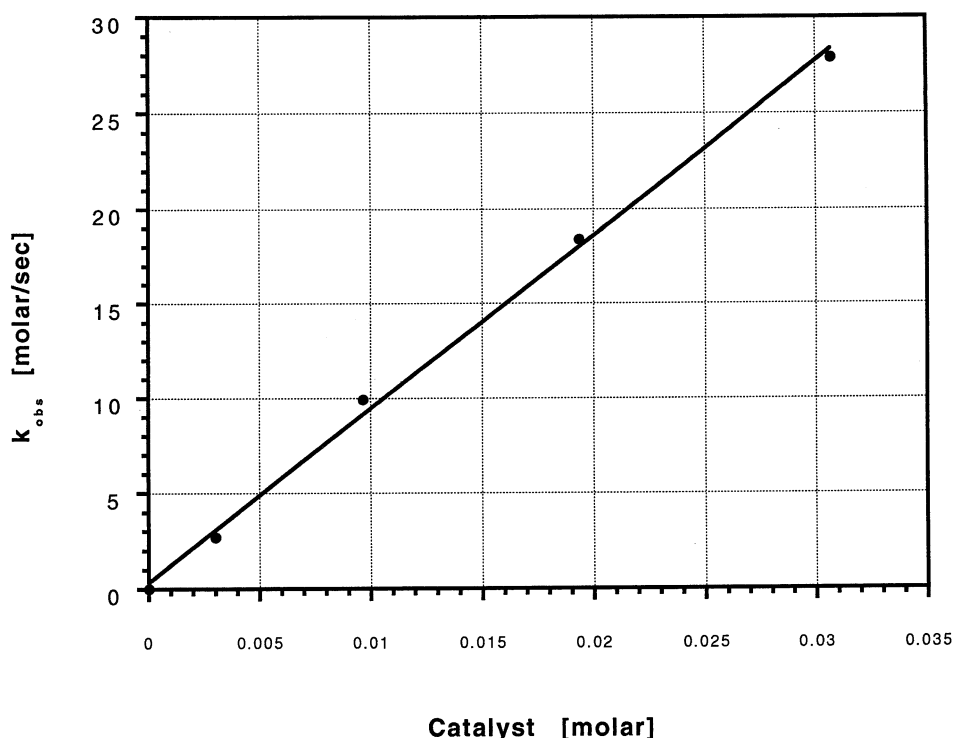
Fig. 2. Determination of the reaction order in [(E_2N)_3U][BPh_4] concentration for the dimerization of nBuC\equiv CH in benzene- d_6 at 25^\circ C .
