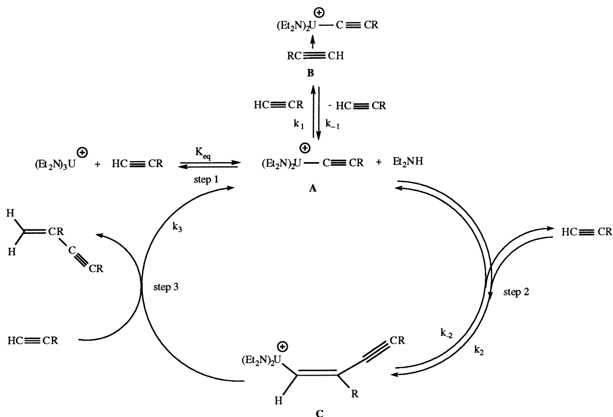
Scheme 2. Plausible mechanism for the dimerization of terminal alkynes promoted by [(Et_2N)_3U][BPh_4] .
