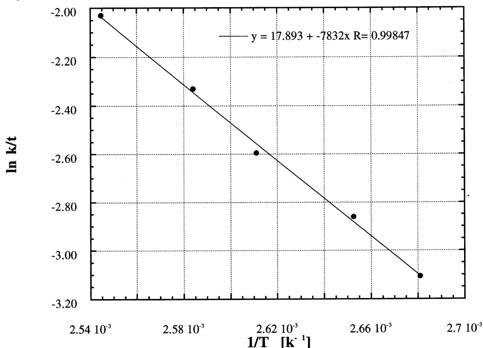
Fig. 4. Eyring plot for the dimerization of n BuC≡CH using [(E 2 N) 3 U][BPh 4 ] as the precatalyst in toluene- d 8 . This line represents the least-squares fit to the data points.
