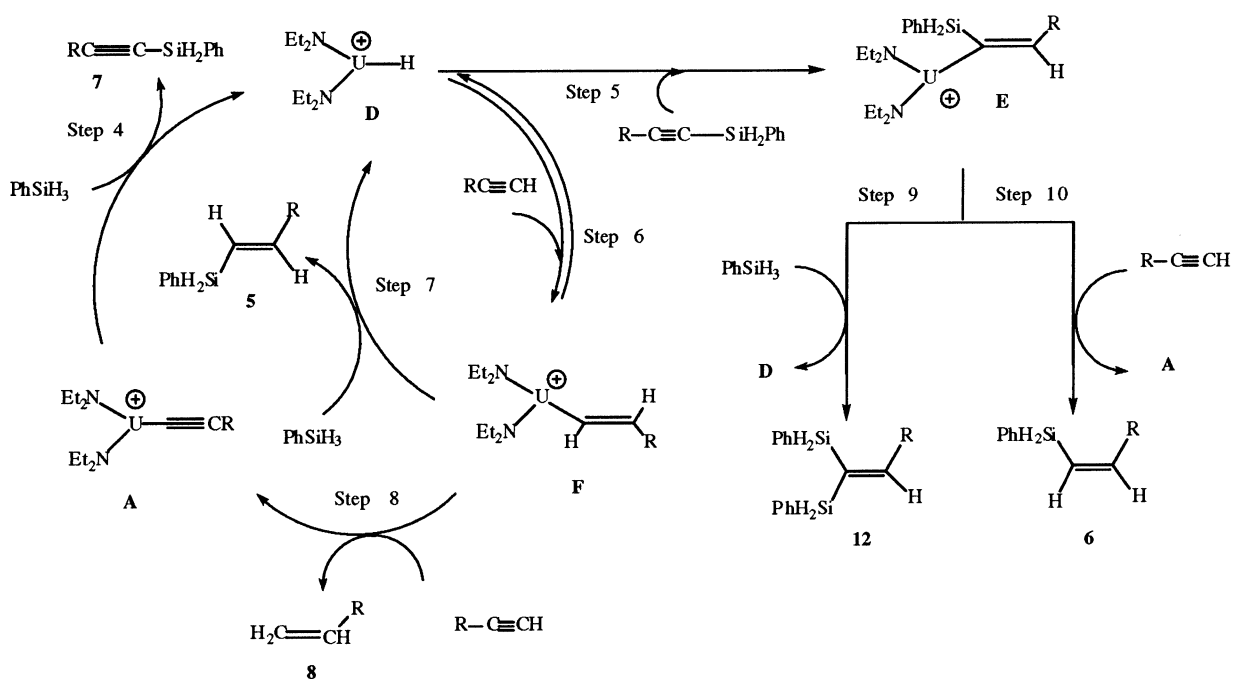
Scheme 3. Plausible mechanism for the room and high temperature hydrosilylation of terminal alkynes promoted by [(Et_2N)_3U][BPh_4] . The transformation of the starting complex into the acetylide complex [(Et_2N)_2U-C\equiv CR][BPh_4] ( A ) was described in Scheme 2, and is omitted here for clarity.
