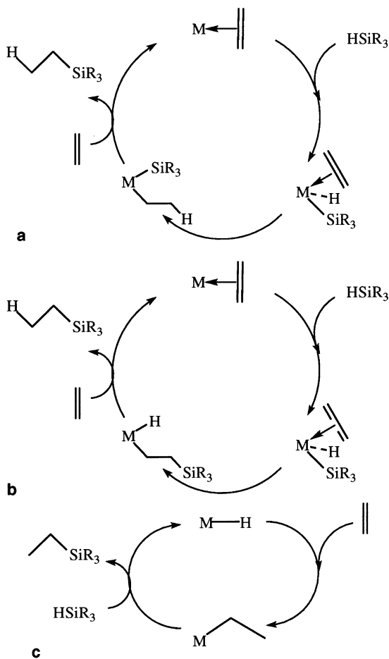
Scheme 1. Proposed mechanisms for the hydrosilylation of alkenes: Chalk–Harrod (1a), modified Chalk–Harrod (1b) and modified Chalk–Harrod for early-transition metal complexes (1c).
