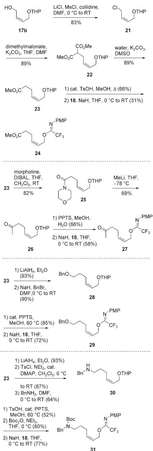
Scheme 4. Preparation of functionalized substrates 24 , 27 , 29 and 31 .
