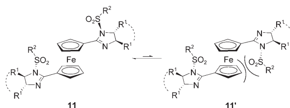
Figure 2. Chirality transfer to the sulfonylated N-atoms as major ligand design principle resulting in a preferred equilibrium conformation of 11 to allow for a highly diastereoselective biscyclopalladation.
