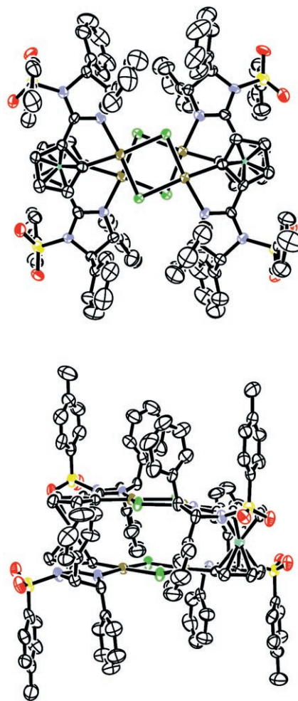
Figure 3. Ortep-representations of the dimeric bispalladacycle 12a . The 30 % probability ellipsoids have the following color code: C (black); N (blue); O (red); S (yellow); Fe (aquamarine); Pd (bronze); Cl (green). H atoms are omitted for clarity. At the top: view along the ferrocene axis; below: view perpendicular to the ferrocene axis.
