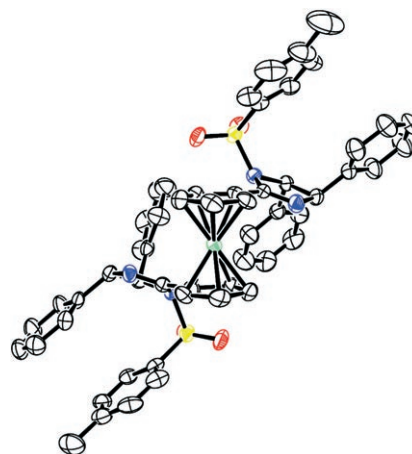
Figure 1. ORTEP representation of ligand 11a (R 2 = p -Tol). The 30% probability ellipsoids have the following color code: C (black); N (blue); O (red); S (yellow); Fe (aquamarine). H atoms are omitted for clarity.
