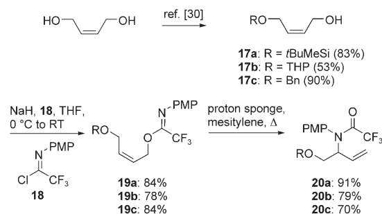
Scheme 3. Preparation of functionalized substrates 19a–c .
