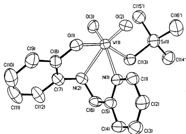
Figure 1. Molecular structure of WO 2 (L 1 )(CH 2 SiMe 3 ). Selected bond lengths (Å) and angles (deg) are as follows: W(1)–O(1) = 1.986(4), W(1)–O(2) = 1.709(4), W(1)–O(3) = 1.711(4), W(1)–N(1) = 2.333(4), W(1)–N(2) = 2.369(4), W(1)–C(13) = 2.149(6); O(1)–W(1)–O(2) = 97.66(18), O(1)–W(1)–O(3) = 100.89(17), O(2)–W(1)–O(3) = 106.96(19), O(1)–W(1)–N(1) = 78.87(15), O(2)–W(1)–N(1) = 89.11(16), O(3)–W(1)–N(1) = 163.73(18), O(1)–W(1)–N(2) = 74.27(16), O(2)–W(1)–N(2) = 157.53(16), O(3)–W(1)–N(2) = 95.25(17), N(1)–W(1)–N(2) = 68.89(12), O(1)–W(1)–C(13) = 154.13(19), O(2)–W(1)–C(13) = 98.6(2), O(3)–W(1)–C(13) = 93.5(2), N(1)–W(1)–C(13) = 81.38(18), N(2)–W(1)–C(13) = 83.12(19), W(1)–C(13)–Si(1) = 116.8(3).
