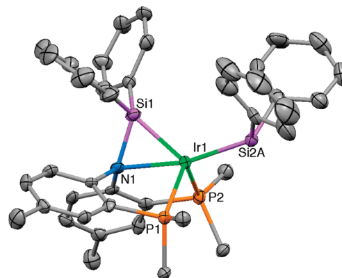
Figure 4. Molecular structure of the cation in 20 , displaying thermal ellipsoids at the 50% probability level. H-atoms, the carborane anion, and Si2B have been omitted for clarity. Selected bond lengths (Å): Ir1–Si1 = 2.318(2), Ir1–Si2A = 2.365(2), Ir1–N1 = 2.294(4), N1–Si1 = 1.795(5). Selected angles (deg): P1–Ir1–P2 = 102.39(5), Si1–Ir1–Si2A = 121.01(6), N1–Ir1–Si1 = 45.8(1).
