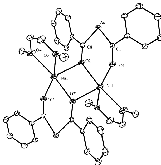
Fig. 4 Molecular structure of compound 9 . Selected bond lengths (Å) and angles (°): As(1)–C(8) 1.916(3), As(1)–C(1) 1.939(3), O(1)–C(1) 1.242(4), O(2)–C(8) 1.248(4), O(1)–Na(1) 2.201(3), O(2)–Na(1) 2.261(3), Na(1)–O(4) 2.295(3), Na(1)–O(2) 2.342(4), Na(1)–O(3) 2.554(17), C(8)–As(1)–C(1) 101.24(14), O(1)–C(1)–As(1) 127.6(3), O(2)–C(8)–As(1) 127.1(3), C(8)–O(2)–Na(1) 120.4(3), C(8)–O(2)–Na(1) 120.4(3), C(1)–O(1)–Na(1) 140.3(3), O(1)–Na(1)–O(2) 110.08(14), O(2)–Na(1)–O(2) 89.17(12). Symmetry operation i : – x , – y + 1, – z .
