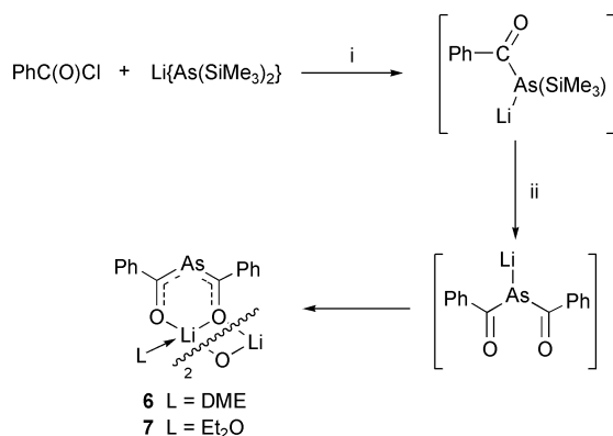
Scheme 2 Reagents and conditions: (i) DME, -\text{SiMe}_3\text{Cl} ; (ii) \text{PhC(O)Cl} , -\text{SiMe}_3\text{Cl} .
