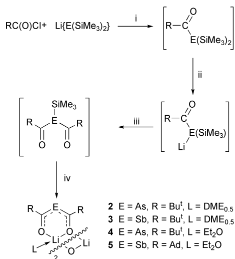
Scheme 1 Reagents and conditions: (i) DME, -\text{LiCl} ; (ii) \text{Li}\{\text{E}(\text{SiMe}_3)_2\} , -\text{E}(\text{SiMe}_3)_3 ; (iii) \text{RC(O)Cl} , -\text{LiCl} ; (iv) \text{Li}\{\text{E}(\text{SiMe}_3)_2\} , -\text{E}(\text{SiMe}_3)_3 .
