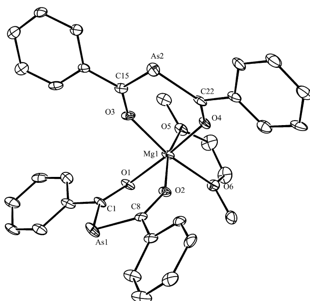
Fig. 7 Molecular structure of compound 12 . Selected bond lengths (Å) and angles (°): As(1)–C(8) 1.916(10), As(1)–C(1) 1.938(9), As(2)–C(15) 1.908(10), As(2)–C(22) 1.928(9), Mg(1)–O(3) 2.000(6), Mg(1)–O(2) 2.007(6), Mg(1)–O(4) 2.028(7), Mg(1)–O(1) 2.029(7), Mg(1)–O(6) 2.129(6), Mg(1)–O(5) 2.131(6), O(1)–C(1) 1.253(9), O(2)–C(8) 1.251(10), O(4)–C(22) 1.261(9), O(3)–C(15) 1.250(9), C(8)–As(1)–C(1) 99.1(4), O(3)–Mg(1)–O(4) 88.5(3), O(2)–Mg(1)–O(1) 88.4(3), O(6)–Mg(1)–O(5) 74.5(3), C(1)–O(1)–Mg(1) 132.3(6), O(1)–C(1)–As(1) 127.6(8), C(15)–As(2)–C(22) 99.2(4), C(8)–O(2)–Mg(1) 137.7(7), C(15)–O(3)–Mg(1) 137.5(7), C(22)–O(4)–Mg(1) 132.0(6), O(2)–C(8)–As(1) 126.8(7), O(3)–C(15)–As(2) 127.2(8), O(4)–C(22)–As(2) 127.6(8).
