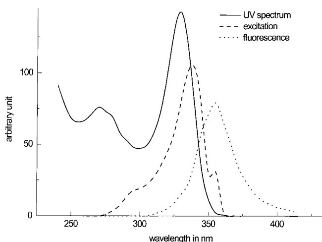
Fig. 2 UV, excitation and fluorescence spectrum of [\text{Hept Si}(\text{CH}_2)_3\text{OPh}] ( 3d ) in n -hexane solution
