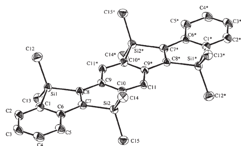
Figure 8. ORTEP drawing of 17 (50% probability for thermal ellipsoids).
