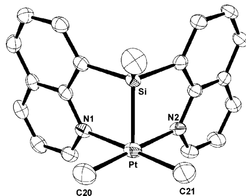
Figure 4. ORTEP diagram of the cationic complex 9 with thermal ellipsoids shown at the 50% probability level. Hydrogen atoms and the \text{B}(\text{C}_6\text{F}_5)_4 anion are omitted for clarity. Selected bond lengths (Å): Pt–Si = 2.256(1), Pt–N1 = 2.142(3), Pt–C20 = 2.036(5). Selected bond angles (deg): C20–Pt–C21 = 90.9(2), N1–Pt–N2 = 91.4(1), Si–Pt–C20 = 95.5(2).
