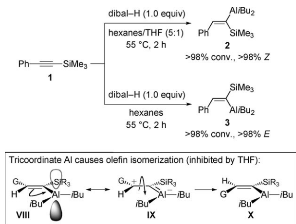
Scheme 3. Stereoselective hydroalumination of trimethylsilylphenylacetylene with dibal-H, and a rationale for the effect of a Lewis base (THF). dibal-H = ( i Bu) 2 AlH.
