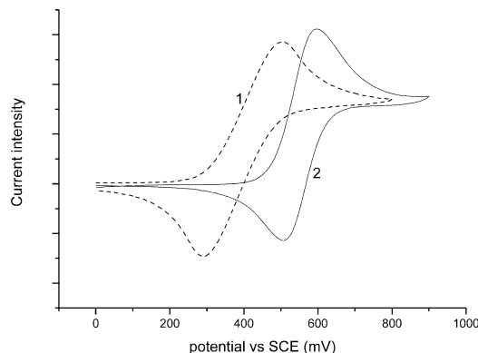
Figure 1. Cyclic voltammetry of the oxidation of a solution of 1 (---) in DME and of a solution of 2 in THF (—).
