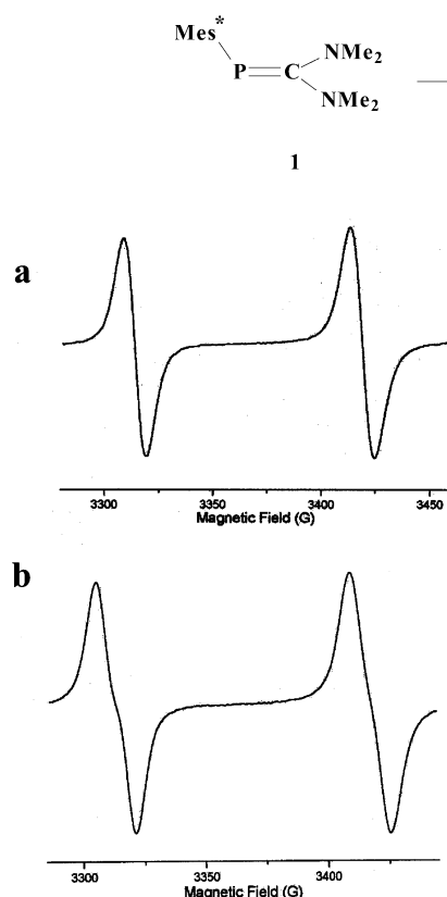
Figure 2. EPR spectra obtained at room temperature by electrochemical oxidation of (a) a solution of 1 in THF and (b) a solution of 1 - 13 C, d 12 in THF.
