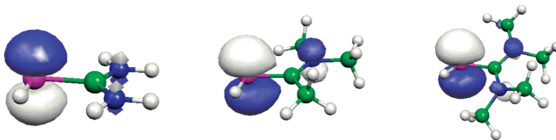
Figure 5. Representation of the SOMO for \mathbf{M3}^{\bullet+} , \mathbf{M2}^{\bullet+} , and \mathbf{M4}^{\bullet+} .
