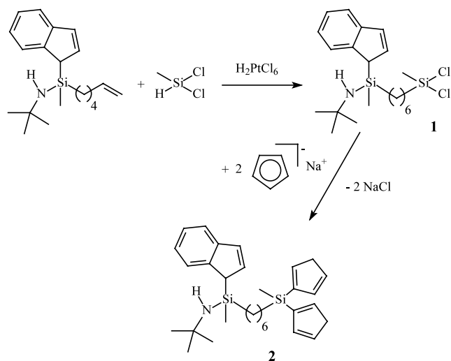
Scheme 1. Synthesis of the intermediate 1 and the ligand precursor 2 .
