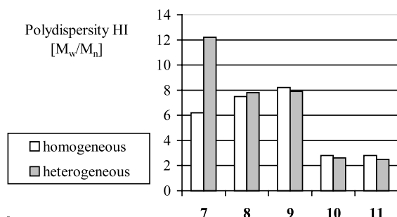
Scheme 7. Polydispersities HI of the polyethylenes obtained from 7–11/MAO.
