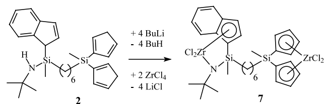
Scheme 2. Synthesis of the dinuclear complex 7 .
