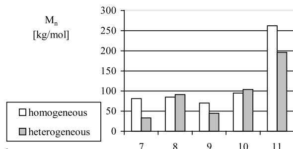
Scheme 6. Molecular weights M_n of the polyethylenes obtained from 7–11/MAO.
