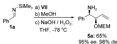
Scheme 3. Alkoxyallylboration of N-silylimines.
