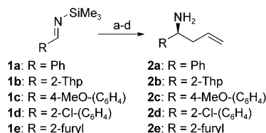
Scheme 1. Allylboration of N-silylimines: a) I , THF; -100 or -78^\circ\text{C} ; b) 1a–e ; c) \text{H}_2\text{O} ; 1 h, -100 or -78^\circ\text{C} ; d) \text{NaOH} , \text{H}_2\text{O}_2 ; -78^\circ\text{C} \rightarrow \text{RT} . Thp = thiophene.
