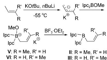
Figure 2. Preparation of reagents for asymmetric crotylboration. Ipc = isopinocampheyl.
