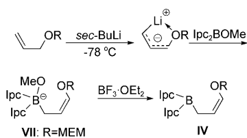
Figure 3. Preparation of alkoxyallylborane reagents.
