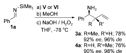
Scheme 2. Crotylboration of N-silylimines.
