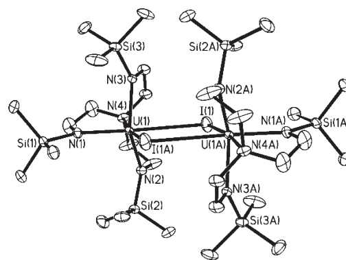
Figure 2. Molecular structure of 3·0.5C 7 H 8 with selective atom labeling and probability ellipsoids set at 30%. Hydrogen atoms and minor iodide disorder components omitted for clarity. Only the major component of the disordered iodide and one of the two unique molecules are shown for clarity. The structure of 3·2C 7 H 8 is very similar.
