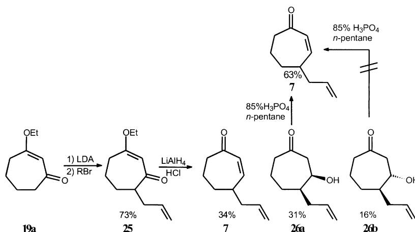
Scheme 9. Synthesis of the 4-substituted derivative 7 .
