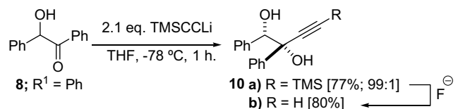
Scheme 3. Condensation of benzoin [ 8 ; \text{R}^1 = \text{Ph} ] with TMS acetylene.
