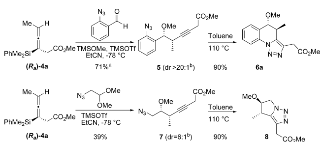
Scheme 1. Two-Step Triazole Formation a,b
