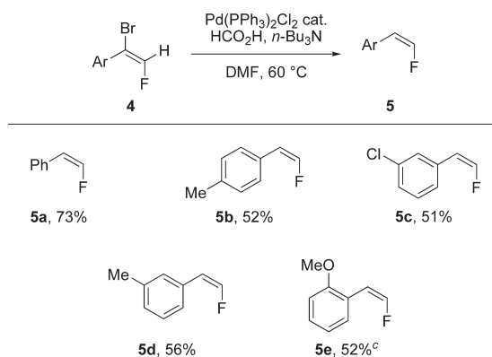
Scheme 4. Synthesis of cis - \beta -Fluorostyrene Derivatives a,b
