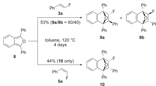
Scheme 5. Diels–Alder of Both Isomers of \beta -Fluorostyrene with 1,3-Diphenylisobenzofuran
