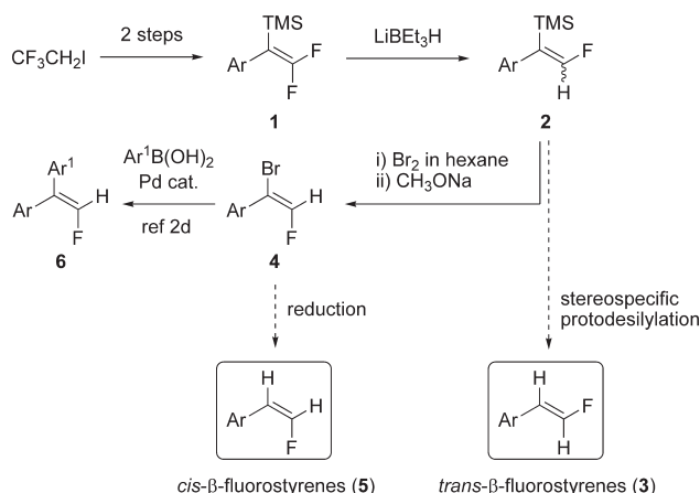
Scheme 1. Stereoselective Approaches to Both Isomers of \beta -Fluorostyrenes
