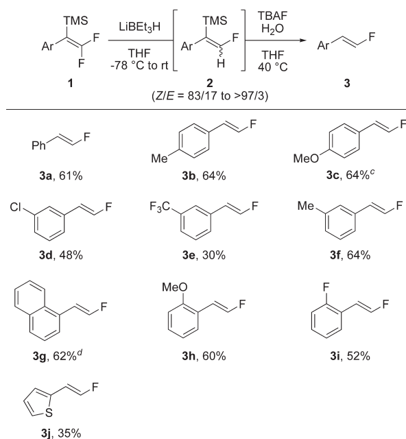
Scheme 2. Synthesis of trans - \beta -Fluorostyrene Derivatives a,b
