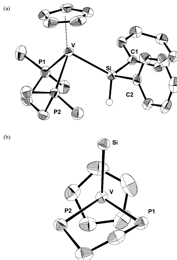
Figure 1. ORTEP drawings of \text{Cp}(\text{dmpe})\text{VSiHPh}_2 ( 2 ), with thermal ellipsoids drawn at the 50% probability level: (a) general view with hydrogen atoms, except for those on the silicon atom, omitted for clarity; (b) view along the V–Cp(centroid) axis with groups on the Si and P atoms removed for clarity. Selected bond distances (Å) and angles (deg): V–Si = 2.5629(8), V–P2 = 2.4621(8), V–P1 = 2.4613(8), Si–H = 1.45(3), Si–C1 = 1.915(2), Si–C2 = 1.913(2), V–Cp(centroid) = 1.946; P1–V–P2 = 81.68(3), P2–V–Si = 87.67(3), P1–V–Si = 92.82(3), V–Si–H = 115(1), V–Si–C1 = 116.93(8), V–Si–C2 = 117.55(8).
