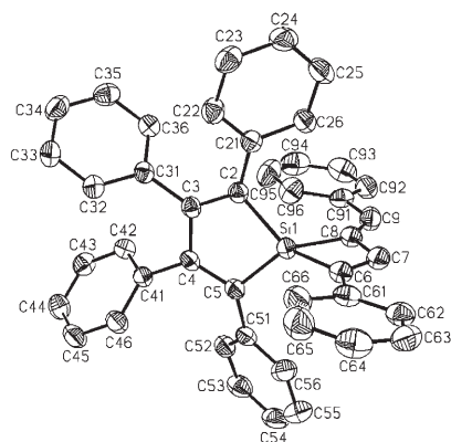
Figure 1. Molecular Structure of 6 . Ellipsoids are drawn at 50 % probability. Hydrogen atoms are omitted for clarity. Selected bond lengths [Å] and angles [°]: Si1–C2 1.871(2), Si1–C5 1.874(2), Si1–C6 1.888(2), Si1–C8 1.888(2), C2–C3 1.357(3), C3–C4 1.515(3), C4–C5 1.360(3), C6–C7 1.343(3), C7–C8 1.452(3), C8–C9 1.332(3); C2–Si1–C5 93.08(9), C6–Si1–C8 74.35(10), Si1–C2–C3 107.14(14), Si1–C5–C4 107.06(14), C2–C3–C4 116.39(17), C3–C4–C5 116.19(17), Si1–C6–C7 89.68(15), Si1–C8–C7 86.55(14), C6–C7–C8 109.4(2), C7–C8–C9 130.4(2).
