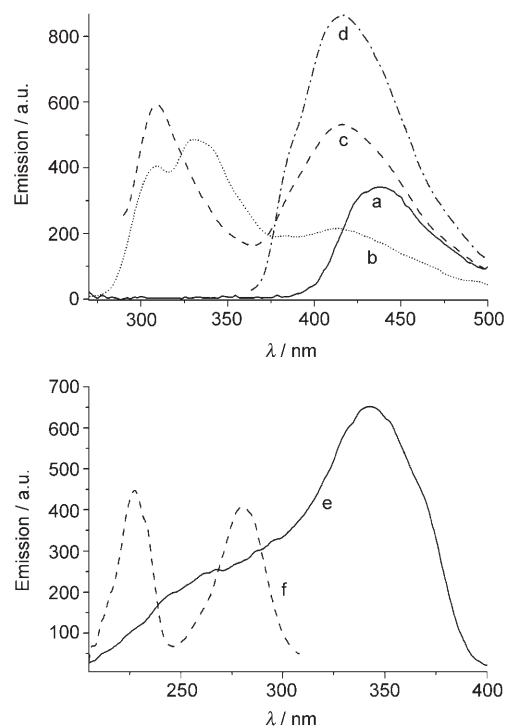
Figure 7. Photoluminescence spectra of silaspiroene 7 and its photoreaction product 15 . a) Solid-state emission spectrum of 7 ( \lambda_{\text{ex}}=260 nm), b) emission spectrum of a solution of silaspiroene 15 in THF ( \lambda_{\text{ex}}=228 nm), c) emission spectrum of a solution of 15 in THF ( \lambda_{\text{ex}}=280 nm), d) emission spectrum of a solution of 15 in THF ( \lambda_{\text{ex}}=344 nm), e) excitation spectrum of a solution of 15 in THF ( \lambda_{\text{fixed}}=416 nm), and f) excitation spectrum of a solution of 15 in THF ( \lambda_{\text{fixed}}=325 nm).
