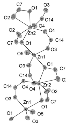
Figure 1. Zinc-oxo chain of Si4A-Zn with 50% probability level thermal ellipsoids.
