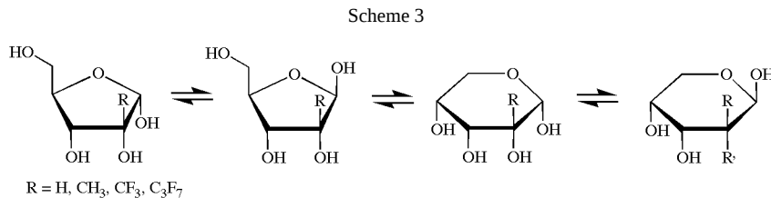
Tautomeric forms of 5 and 10 at equilibrium in acetone- \text{d}_6 at room temperature.
