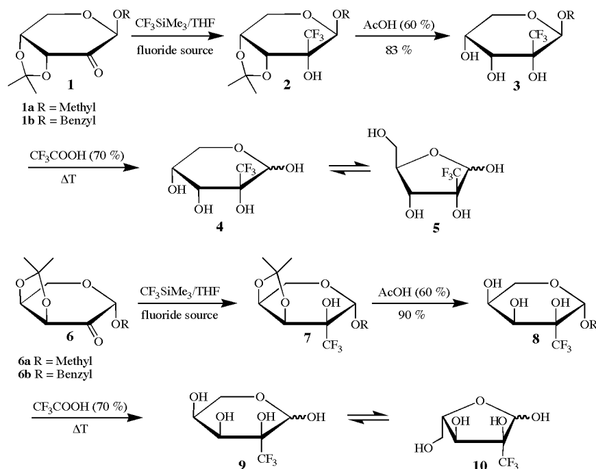
Synthesis of 2-C-trifluoromethyl-D-ribose ( 5 ) and L-ribose ( 10 ).
