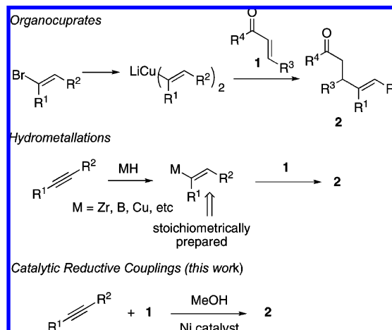
Scheme 1. Progression of Strategies for Effecting Conjugate Addition
