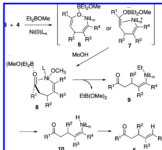
Scheme 2. Mechanism of Triethylborane-Mediated Reductive Couplings
