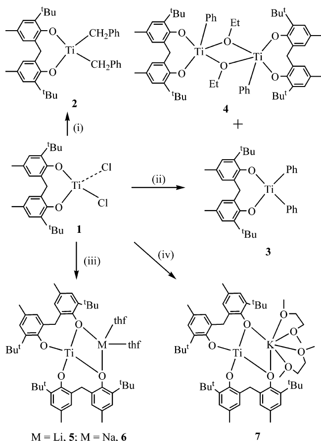
Scheme 1. Synthesis of Titanium Complexes 2–7 a
