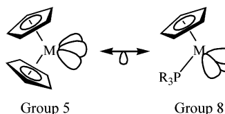
Chart 5. Isolobal Relationship between Group 5 Fragment Cp 2 M and Group 8 Fragment Cp(R 3 P)M
