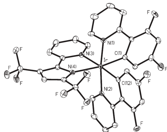
Fig. 1 ORTEP diagram of Flrfpy with thermal ellipsoids shown at 50% probability level; bond distances: Ir–N(1) = 2.046(3), Ir–N(2) = 2.053(3), Ir–N(3) = 2.144(3), Ir–N(4) = 2.155(3), Ir–C(1) = 2.006(3), Ir–C(12) = 2.004(4) Å.
