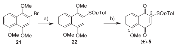
Scheme 5. Synthesis of ( \pm )-5-methoxy-2-( p -tolylsulfinyl)-1,4-naphthoquinone ( 5 ): a) n BuLi, THF, -78^{\circ}\text{C} ; then MeOSOpTol, -78^{\circ}\text{C} , 2 h, 65%; b) CAN, MeCN, \text{H}_2\text{O} , RT, 1 h, 79%.
