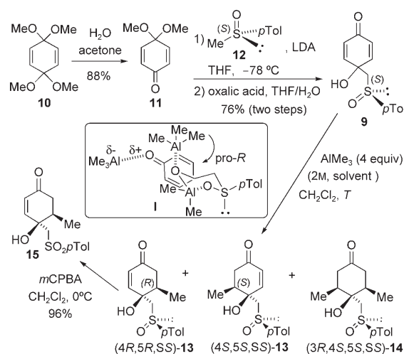
Scheme 2. Synthesis of β-hydroxy sulfone 15 from p -benzoquinone dimethyl ketal 10 .
