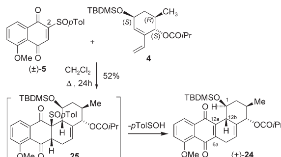
Scheme 7. Diels–Alder reaction between diene 4 and ( \pm )-5-methoxy-2-( p -tolylsulfinyl)-1,4-naphthoquinone ( 5 ).
