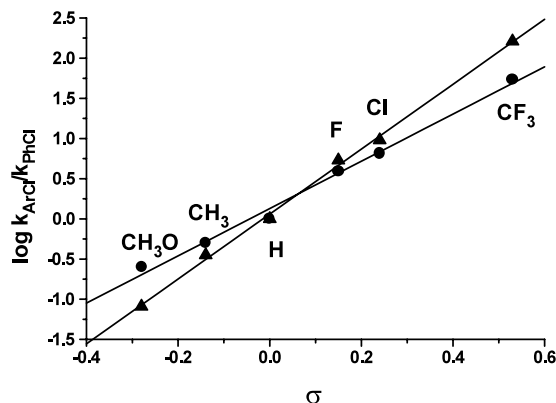
Fig. 1. Hammett plots for the reactions of \text{Me}_3\text{Sn}^- (▲) and \text{Me}_3\text{Si}^- (●) ions with \text{ArX} in HMPA.
