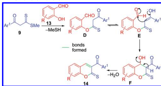
SCHEME 6. Plausible Mechanism for the Synthesis of 2H-Chromene-2-thiones 14
