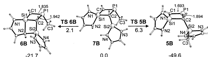
Figure 3. Relative SCS-MP2/6-311 + G**//B3LYP/6-31G* energies (in kcal mol −1 ) for the rearrangement of 6B to the thermodynamically more stable 5B with selected bond lengths [Å].
