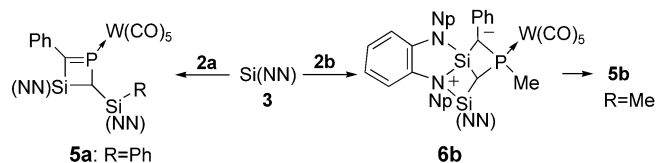
Scheme 1. Synthesis of 2,3-dihydro-1,3-phosphasiletes 5 .
