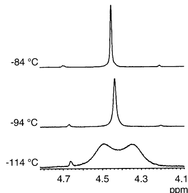
Figure 5. Variable-temperature ^1\text{H} NMR spectra of 8b in \text{THF-}d_8 showing SiH signals.
