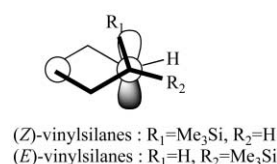
Fig. 6 Orientation of C–Si bond and empty p-orbital in (Z)- and (E)-vinylsilane carbocations.
