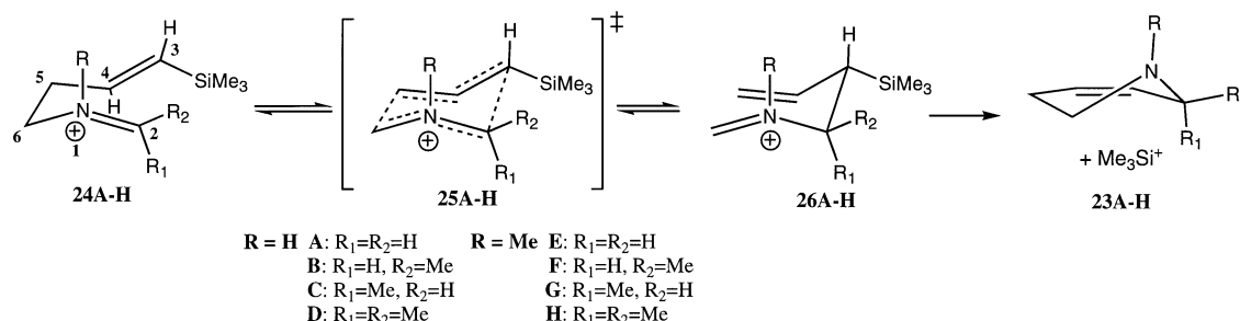
Fig. 5 Calculated mechanism for cyclization of (E)-vinylsilanes.
