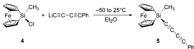
Scheme 4. Synthesis of Ferrocenophane 5 with a Diyne Substituent
