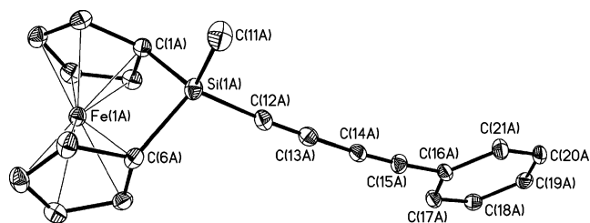
Figure 2. Molecular structure of 5 (thermal ellipsoids at 30% probability). Hydrogen atoms have been removed for clarity, and only one of the two independent molecules of 5 in an asymmetric unit is shown.
