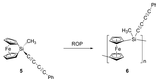
Scheme 5. Ring-Opening Polymerization of Ferrocenophane 5 to Form PFS 6
