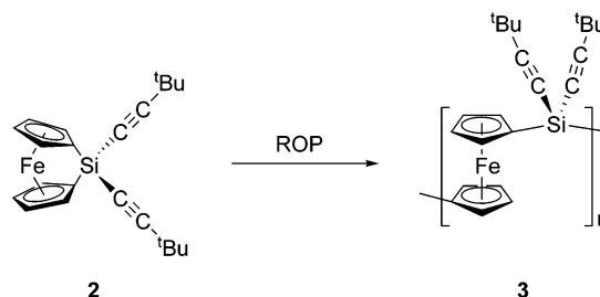
Scheme 2. Ring-Opening Polymerization of Ferrocenophane 2 to Give PFS 3
