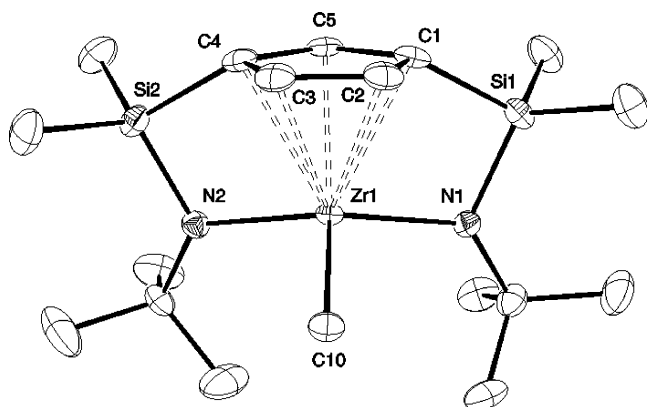
Figure 1. Molecular structure of complex [\text{Zr}\{\eta^5\text{-C}_5\text{H}_3\text{-1,3-(SiMe}_2\text{-}\eta\text{-NtBu)}_2\}\text{Me}] , 6 . Thermal ellipsoids are drawn at the 30% probability level. Hydrogen atoms are omitted for the sake of clarity.
