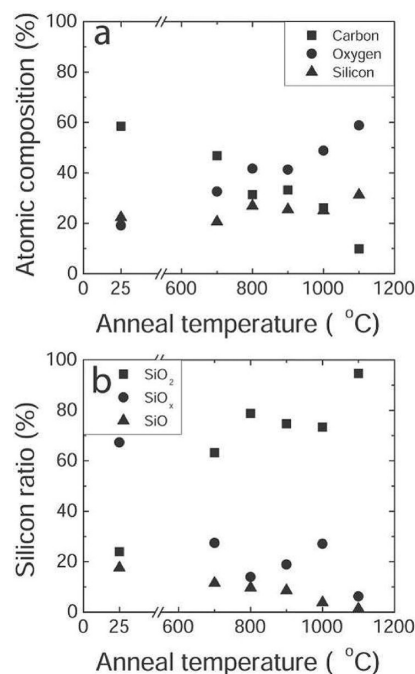
Figure 7. Summary of compositional analyses extracted from the XPS data in Figure 6: (a) relative Si, C, and O content determined by integrating the O 1s, C 1s, and Si 2p peaks; (b) relative \text{SiO} , \text{SiO}_x , and \text{SiO}_2 content determined from the Si 2p peak structure.
