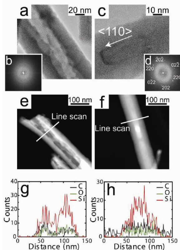
Figure 10. TEM and scanning TEM (STEM) images of Si nanowires annealed at 900 °C under forming gas after 20 electrochemical cycles in a lithium cell. (a, c) Two types of nanowires were observed in nearly equal proportions: (a) amorphous wires that appear to have a hollow core and (c) crystalline nanowires with a thick amorphous shell. (b, d) FFTs of the TEM images in (a) and (c). (e, f) STEM images and (g, h) corresponding EDS line scans at the indicated positions of (e, g) amorphous wires that appear to have a hollow core and (f, h) crystalline nanowires with a thick amorphous shell.
