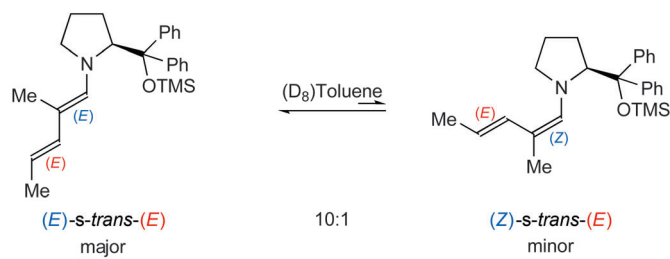
Scheme 3. Comparison of the Conformational Behavior of the Dienamines Formed by Condensation of \alpha -Branched and Linear Enals with Diaryl-prolinol Silyl Ether Derivatives
