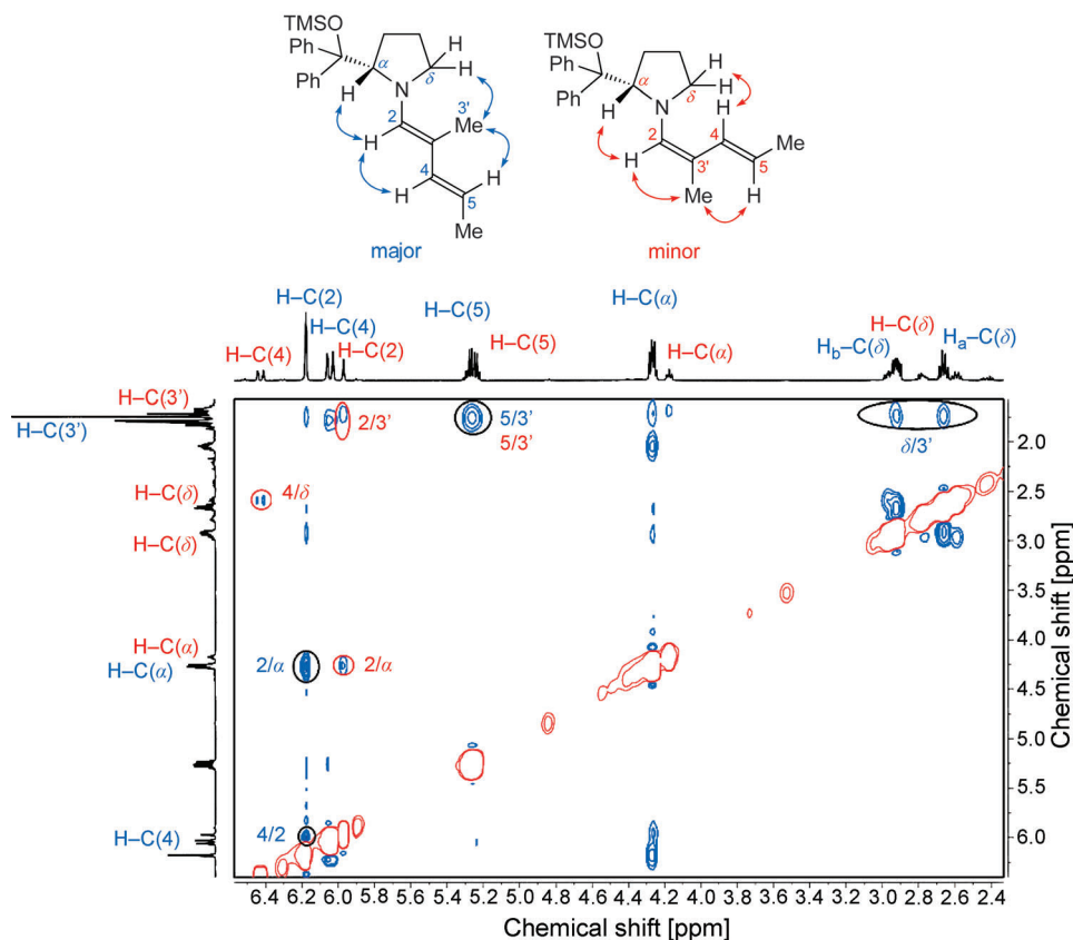
Fig. 3. NOESY Spectra in \text{CDCl}_3 at 298 K
