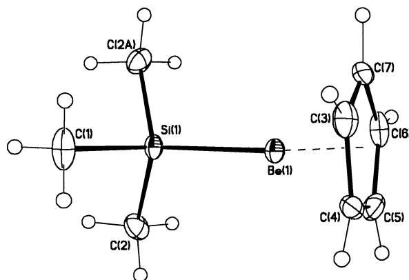
Figure 1. ORTEP drawing of \text{CpBe}(\text{SiMe}_3) , with ellipsoids shown at the 50% level.
