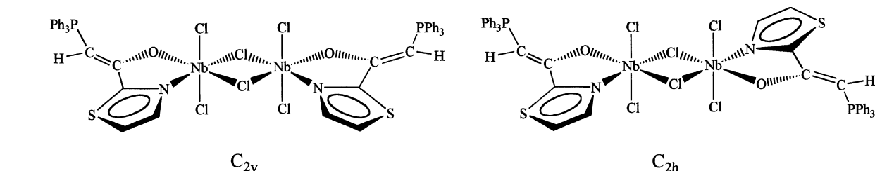
Fig. 1. Proposed structures for complex 1.
