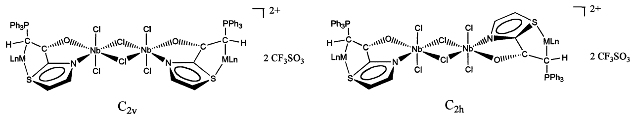
Fig. 4. Proposed structures for complexes 10 – 12 .
