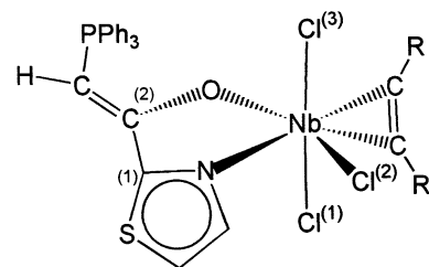
Fig. 2. Proposed structure for complexes 2–8 . Selected bond distances (Å) and angles ( ^\circ ) for complex 7 , from a X-ray crystal structure determination [6]: Nb–O 2.148(3), Nb–N 2.344(5), RC=CR' 1.288(9), Nb–CR 2.066(6), Nb–CR' 2.026(6), O–Nb–N 72.3(1), O–Nb–Cl(2) 159.0(1), Cl(1)–Nb–Cl(3) 161.28(6), CR–Nb–CR' 36.7(2), O–C(2)–C(1) 125.4(5).
