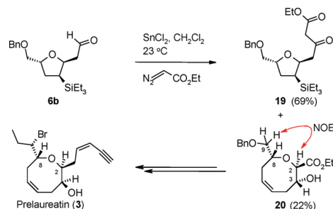
Scheme 5. Synthesis of Oxocene 20
